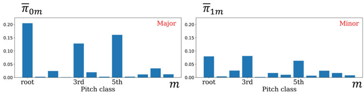
Fig. 5. The emission probabilities \bar{\pi} obtained by the tatum-level model assuming the independence of S .
