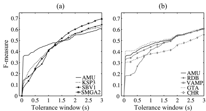
Fig. 8. Evaluation of structural segmentation performance on the RWC-POP database showing F-measure as a function of tolerance window size. (a) AutoMashUpper (AMU) compared to the three unique top performing algorithms in MIREX 2012: SMGA2 [36], KSP3 [35] and SBV1 [37]. (b) AMU compared to different parameterizations. RDB: random downbeat estimates, VAMP: using the QM-VAMP plugin [18] to estimate beat and downbeats, GTA: ground truth beat and downbeat annotations and CHR: using a chromagram for the self-similarity matrix.
