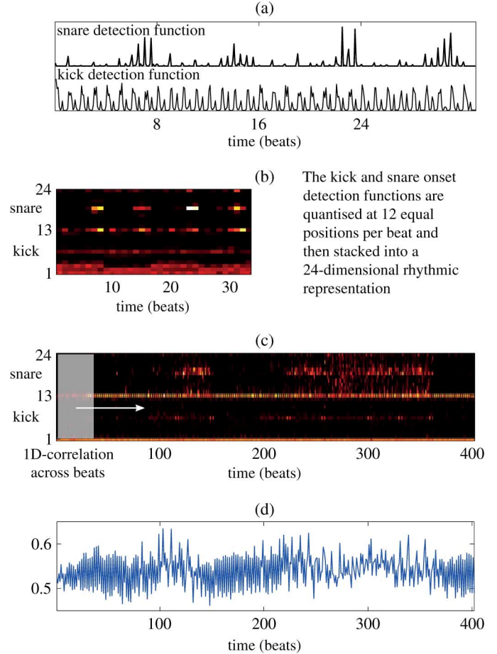
Fig. 4. Rhythmic matching overview. (a) Kick, K_{DF} and snare, S_{DF} , onset detection functions, (b) quantized rhythmic representation for input phrase section, (c) the beat synchronous rhythmic representation for the candidate song, and (d) the rhythmic similarity per beat shift, M_{R,n}(k) .
